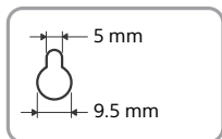
Hole at the rear of the speakers
